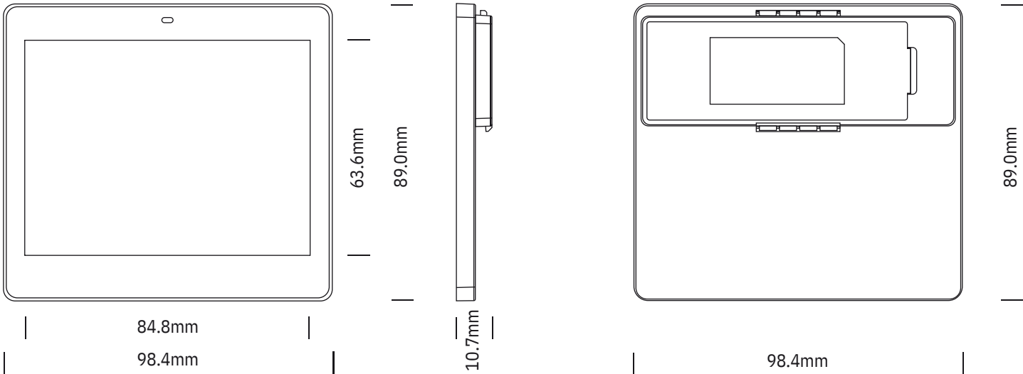
Dimension Drawing
