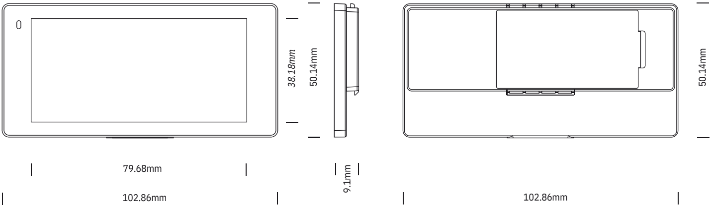
Dimension Drawing
