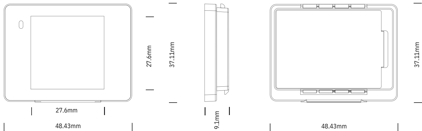
Dimension Drawing
